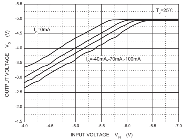
Dropout Characteristics
